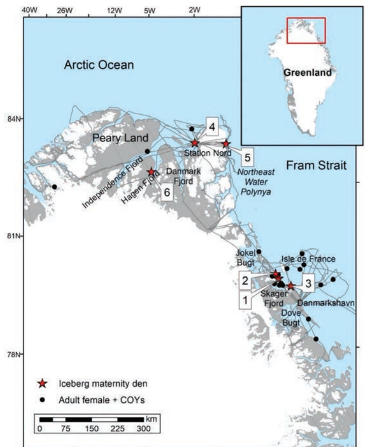
Figure 1. Locations of polar bear maternity dens found in or around grounded icebergs in offshore north and northeast Greenland in April and May 2018 and 2019. Observations or physical captures of family groups (adult females with one or two cubs of the year) are also shown (black dots) with helicopter search tracks (gray lines) flown.
